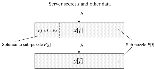
Figure 1. Construction of sub-puzzle P[j]
